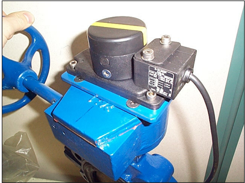
Fig 1.0: Assembly complete with Gearbox
